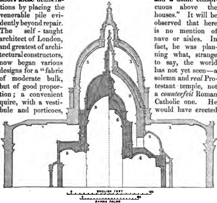
Sections through the transept and dome of St. Peters (1 1 1), Florence Cathedral (2 2), London ditto (3 3), and St. Genevieve, Paris (4 4), showing their comparative widths and heights.
